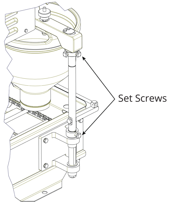
Figure 8 Adjusting the height of the hopper
