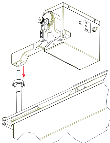
Figure 5 Mounting the cutter head
