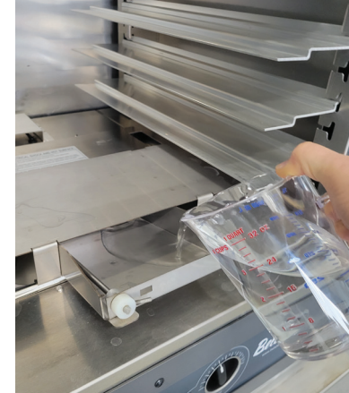
25 Add water to water box
