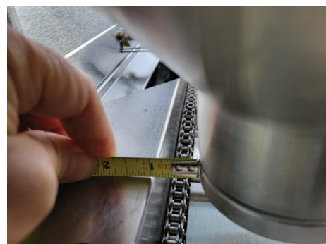
42 Check hopper is 1 inch from side panel
