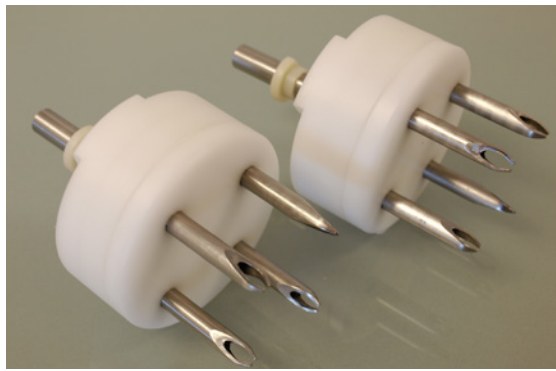
4-Prong spout – Exterior
