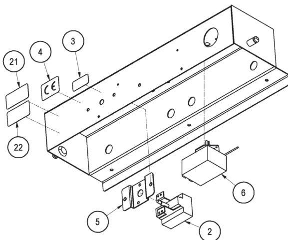
EXPLODED VIEW (INTERNAL BOX COMPONENTS)
