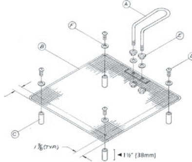
Above: Submerger screen with 1½" spacers (#HP-1004)
